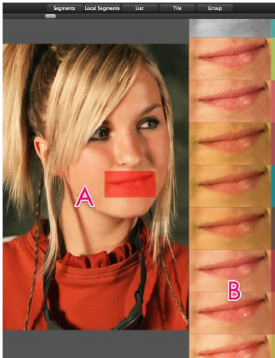
Figure 3: Spatial filter. Users can select particular regions of interest (A), and review the corresponding history via the thumbnail images at (B).
